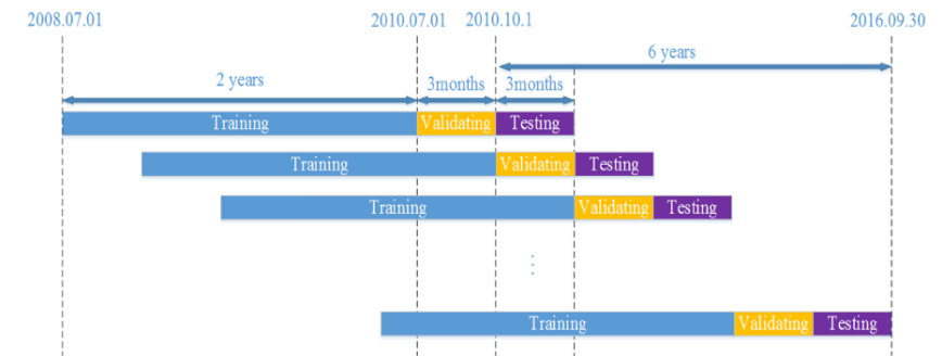
Fig 7. Continuous dataset arrangement for training, validating and testing during the whole sample period.
